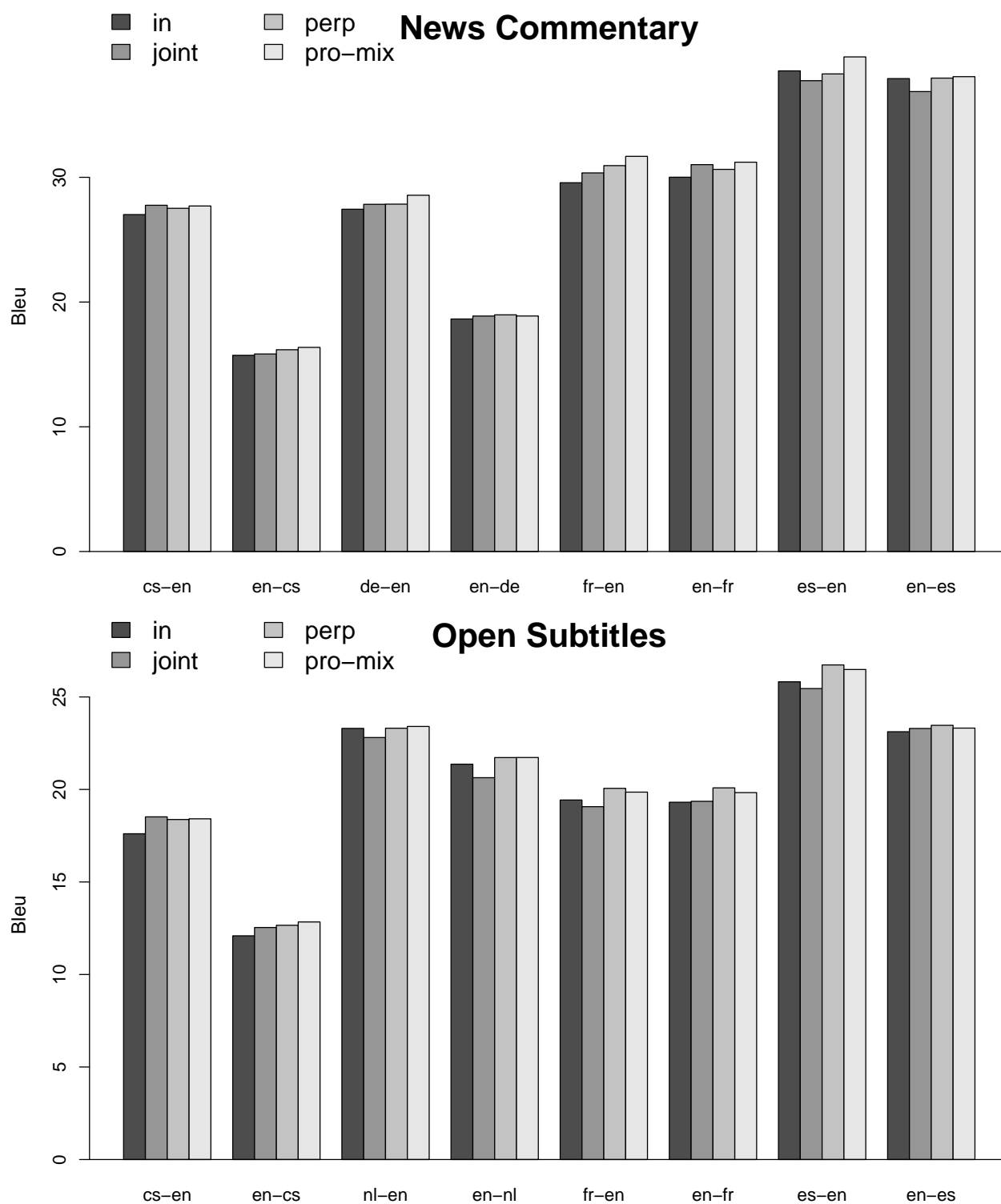
Figure 1: Comparison of the performance (BLEU) on in-domain data, of our pro-mix interpolation weight tuning method with three baselines: in using just in-domain parallel training data training; joint also using europarl data; and perp using perplexity minimisation to interpolate in-domain and europarl data.
