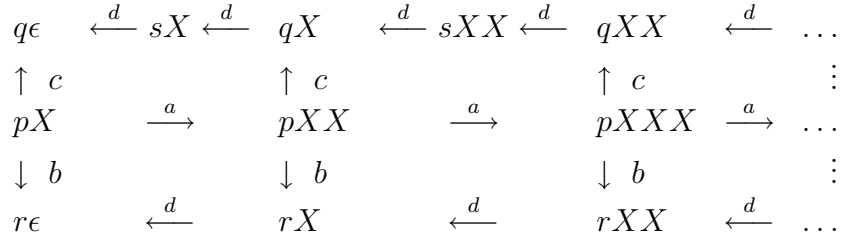
Figure 3: A pushdown automaton
