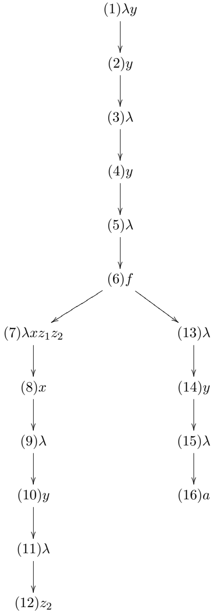
Figure 4: A solution term with order 3 for Example 4.5
