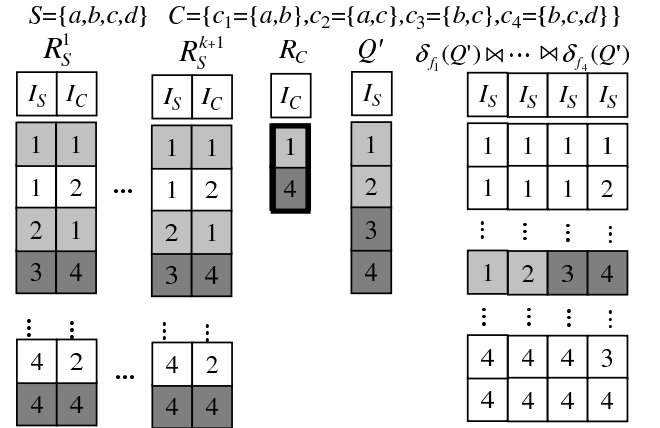
Fig. 7. Illustration of the proof of Theorem 12.
