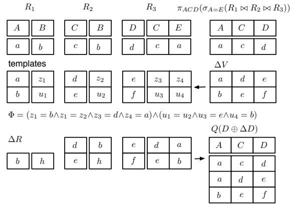
Figure 5: Illustration of the PTIME algorithm in the proof of Theorem 4.4.
