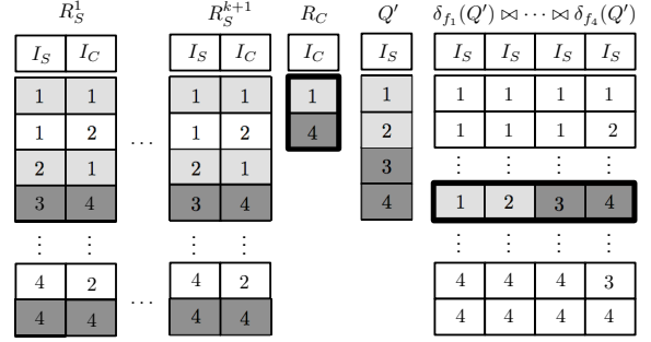
Figure 6: Illustration of the NP-hardness proof of Theorem 4.5.
