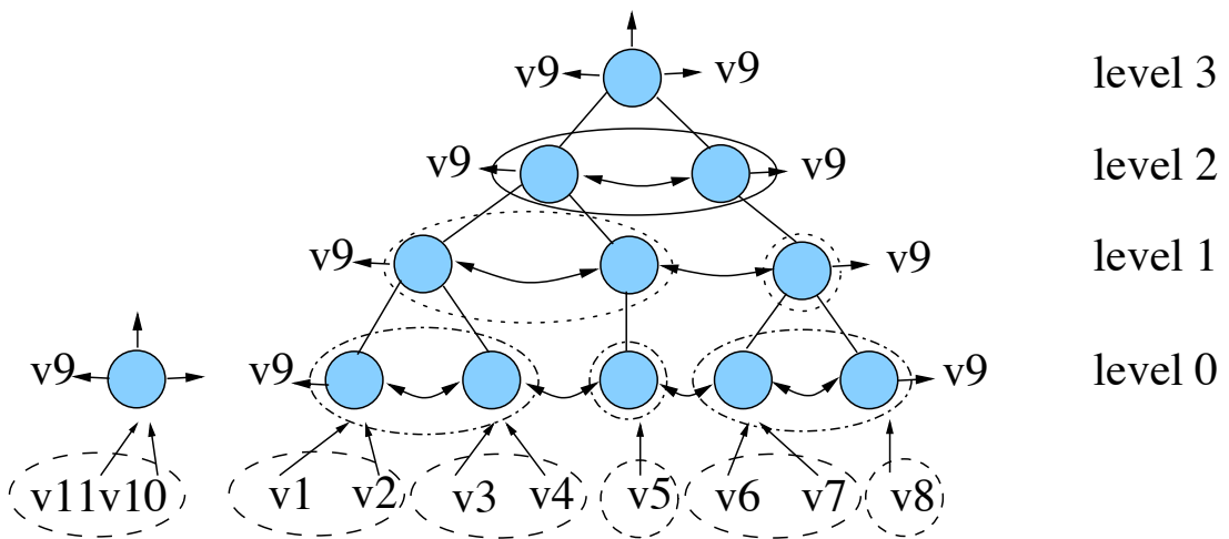
Figure 3: The regular forest corresponding to the regular multilevel partition shown in Figure 2.
