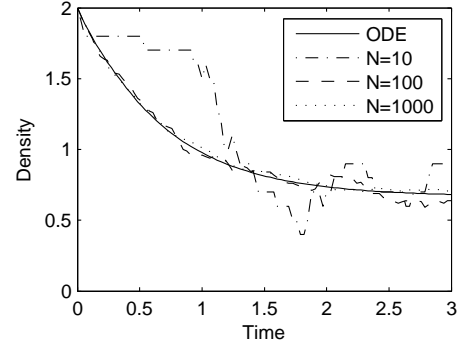
Fig. 1. x_1(t) , i.e., the solution to the ODE (17) giving the time-course evolution of the density of component P in Example 1. One realisation of the scaled Markov chain X_n(t)/n over the first three time units becomes closer to the deterministic estimate as n increases. Parameter set: p = 1.0, p' = 0.5, q = 2.0, q' = 4.0, \delta = (2, 0, 1, 0) .
