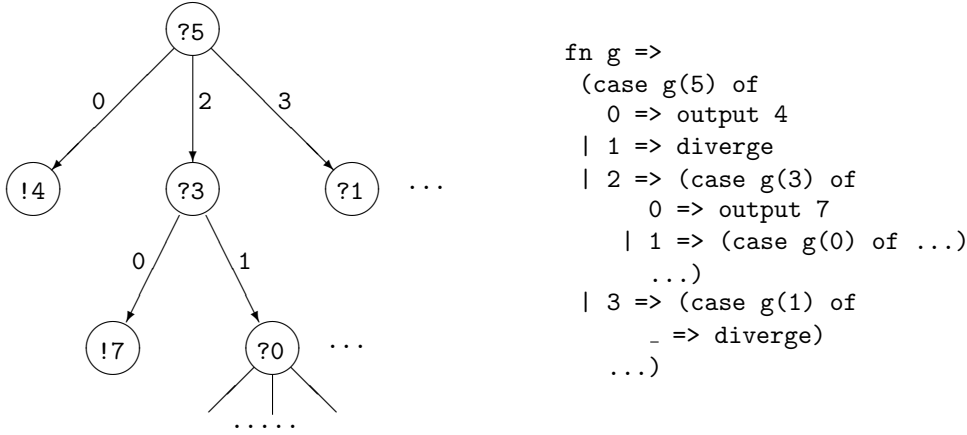
Figure 1: Part of a decision tree for a sequential strategy
