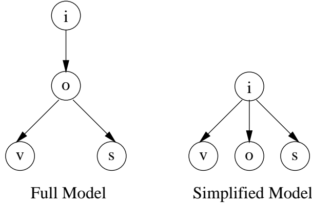
Fig. 1. The two models represented as Bayes nets. Each node is conditionally dependent on all nodes that dominate it.
