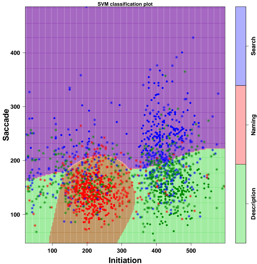
Figure 6. Scatter-plot of Tasks as a function of Mean Saccade Amplitude (pixels), and Initiation Time (ms). The observations are represented as full dots, while the predicted values are represented as asterisks. The three different tasks are color coded as: Description (green), Naming (red), Search (blue). The colored contours represent the SVM classification distributions for the three tasks.
