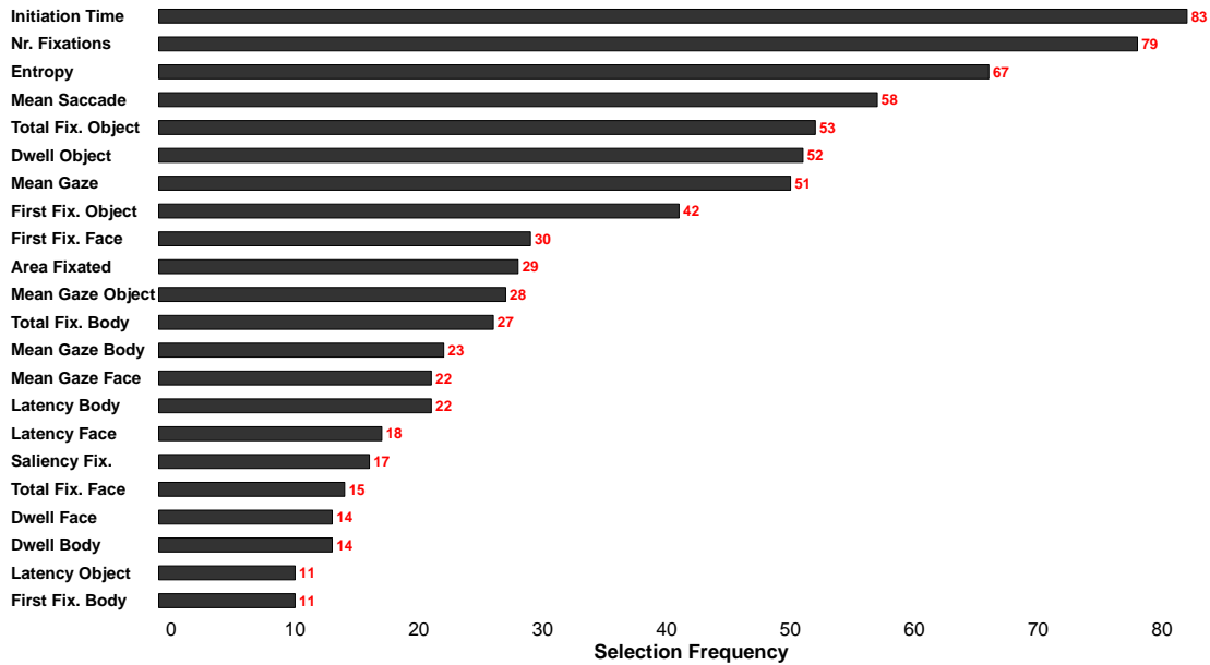
Figure 5. Bar-plot showing the frequency of inclusion of each feature during forward step-wise model selection over ten iterations and ten folds (100 feature sets in total).
