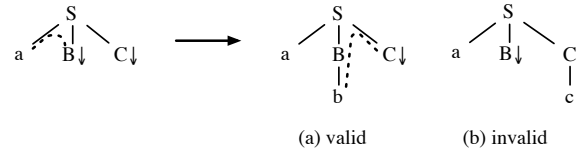
Figure 1: The current fringe (dashed line) indicates where valid substitutions can occur. Other substitutions result in an invalid prefix tree.
