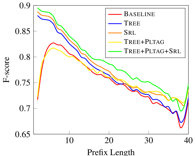
Figure 3: Incremental parsing F-score for increasing sentence prefixes, up to 40 words.
