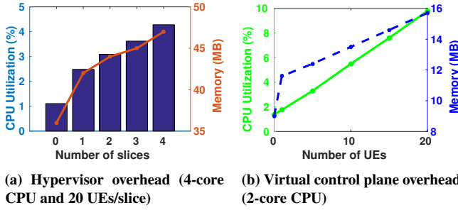
Figure 10: Orion CPU and memory consumption scaling.
