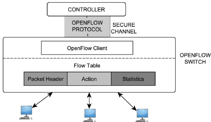
Figure 3.2 Design of an OpenFlow switch and communication with the controller
