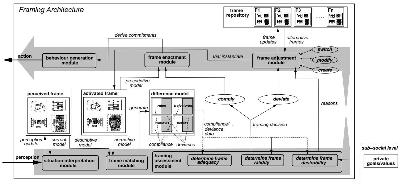
Figure 6: Detailed view of the framing-based agent architecture. The main line of reasoning between perception and action (shown as a shaded arrow) captures both the sub-processes involved and the temporal order in which they occur.
