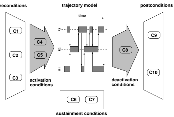
Figure 3: Context model with embedded trajectory that shows conditions C_i in shaded (relevance) and white (enactment) boxes/arrows.
