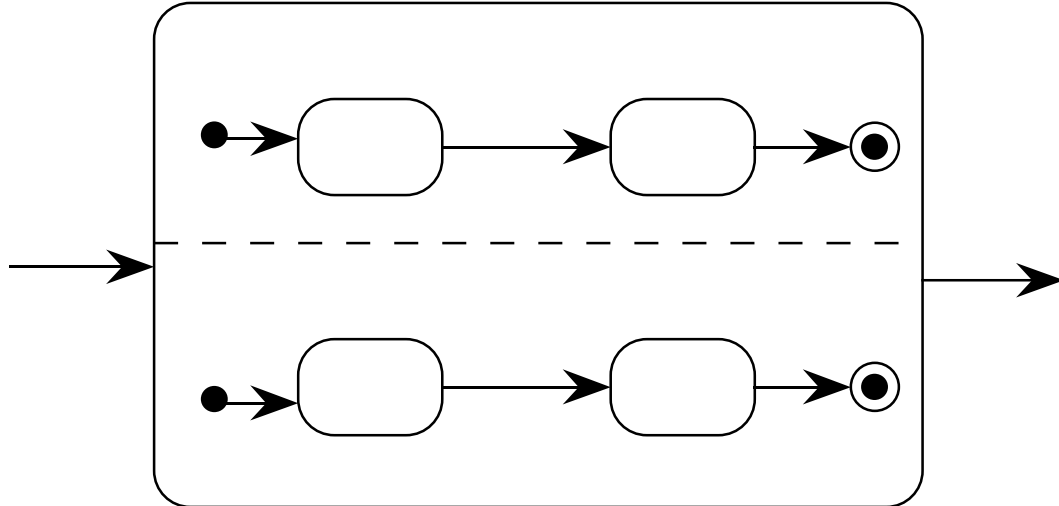
a. State with internal concurrency
