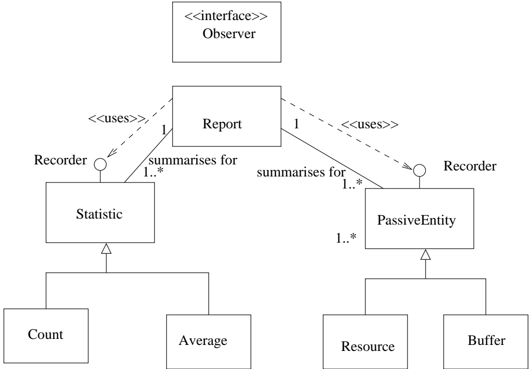
a. Using an interface to show common behaviour
