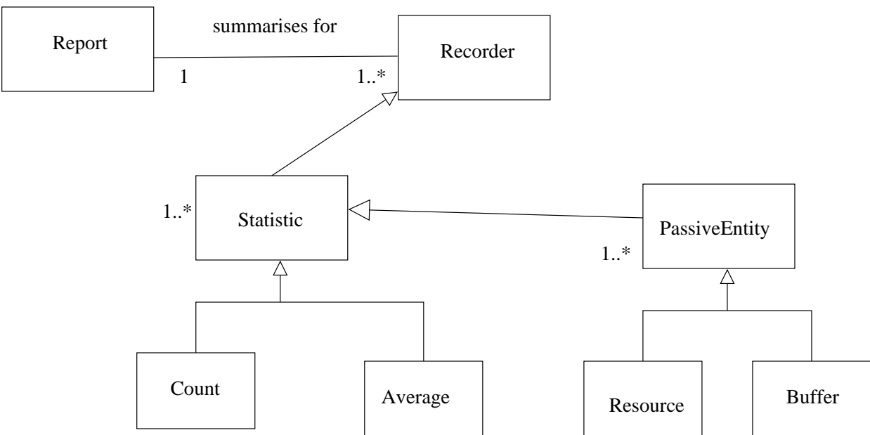
b. One way to use generalisation to show common behaviour
