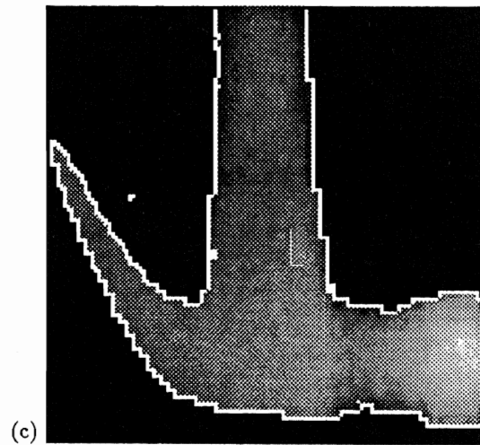
Figure 5: (a) data from a laser range finder for a hammer; (b) its edges using a non-invariant membrane; (c) its edges using an invariant membrane.
