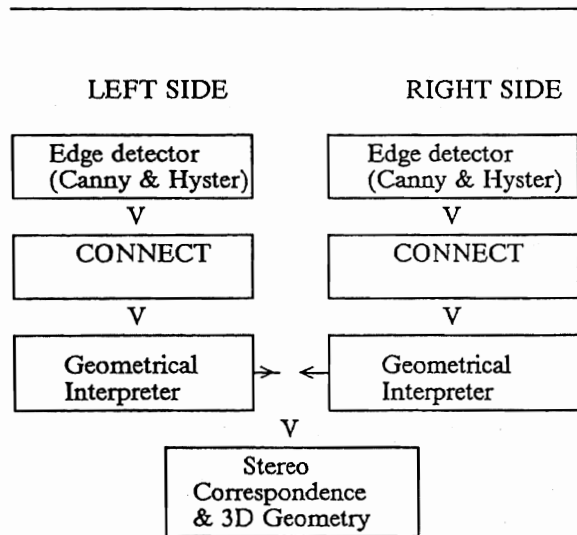
Figure 1. Alternative design of stereo vision system
