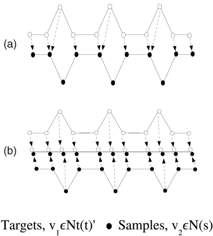
Fig. 6. Point matching via surface projection. (a) Nearest point matching space gives misleading distance-based match metrics. (b) Matching based on common surface projection gives more realistic distance-based match metrics.
