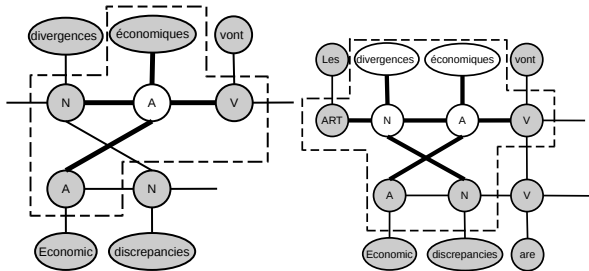
Figure 5: Markov blanket of a tag (left) and of a pair of adjacent tags and words (right).
