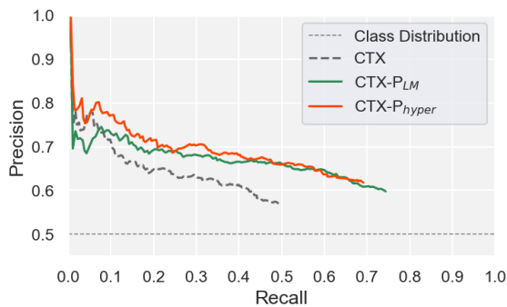
Figure 8: Comparison of P-smoothing methods on ANT: LM-based smoother performs similarly to WordNet hyponym relations on the Entailment Graph CTX.
