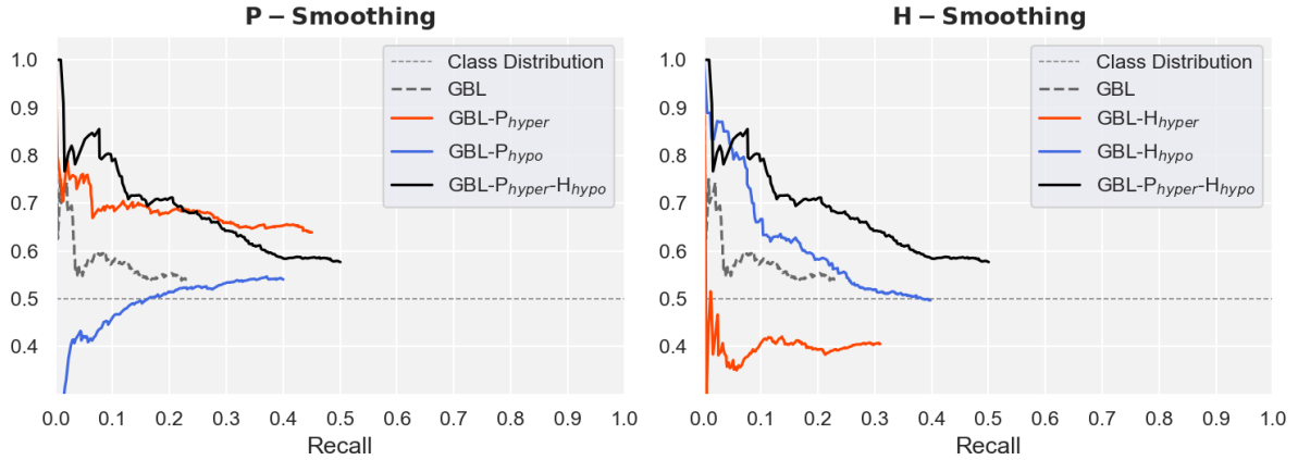
Figure 7: Experiment 3: WordNet relations used to smooth P(\text{remise}) , H(\text{ypothesis}) , and P+H , with the Entailment Graph GBL on the ANT dataset. Hypernyms are useful for P-smoothing, and hyponyms for H-smoothing.
