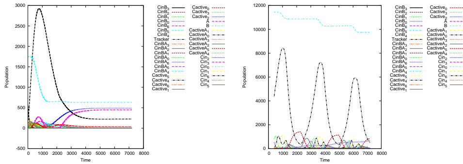
Fig. 6. ODE analysis of the version of the model which has no shortcut reactions. The graph on the left is prior to the optimisation of parameters while the graph on the right is after the optimisation of parameters. Once again parameter optimisation is able to find a configuration in which the model produces an oscillating signal but here the signal appears to dampen.
