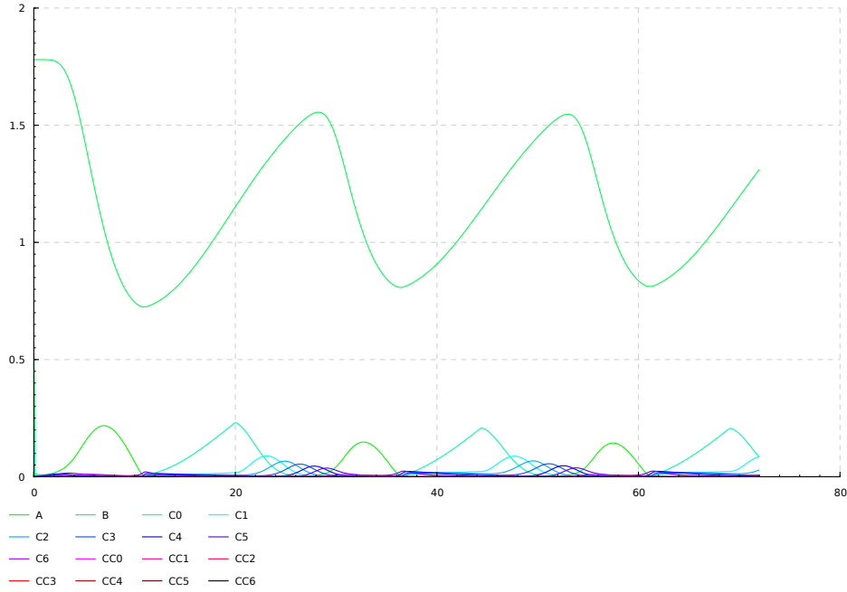
Fig. 7. The time series produced by using CPiWB to generate the ODEs for the Kai system and solving those ODEs using the lsode solver from Gnu Octave. There is a clear oscillating signal.
