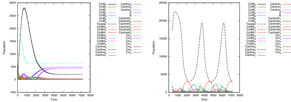
Fig. 4. The graph on the left shows the time course obtained by ODE solution from the full version of the model prior to optimisation of the rate constant parameters. No rhythmic cycle at all is detected. However, once we optimise the rate parameters, as the graph on the right reveals, we can obtain a sustained oscillating signal.
