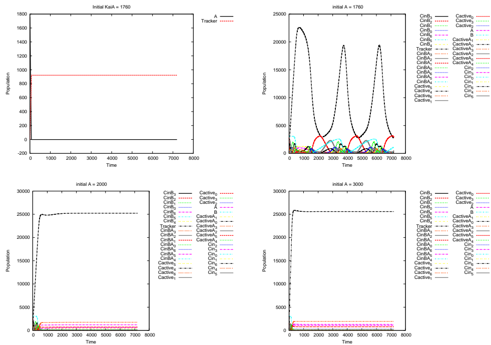
Fig. 5. The graph on the top left shows the full model with optimised parameters evaluated using stochastic simulation and the graph on the top right is the exact same model evaluated via ODEs. We see a startling difference. The graphs on the bottom increase the initial population of the KaiA protein, we see that even a very modest increase removes the oscillation from the signal produced.
