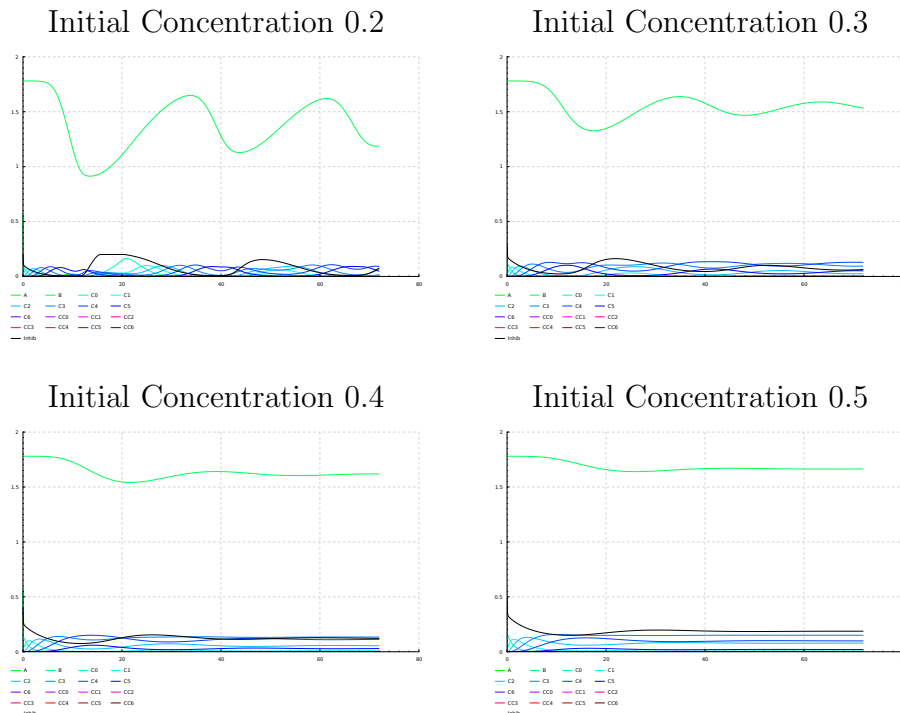
Fig. 9. CPiWB plots of the clock system with the addition of an inhibitor which is an additional agent binding to the KaiA protein and thus preventing the catalysed phosphorylation of the KaiC protein. For each plot we have a different initial concentration of the inhibitor showing that as we increase that initial concentration of the inhibitor the strength of the oscillating signal diminishes.
