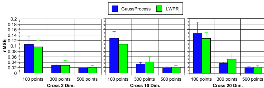
Figure 6: Normalised mean squared error comparisons between LWPR and Gaussian Processes for 2D, 10D and 20D Cross data sets
