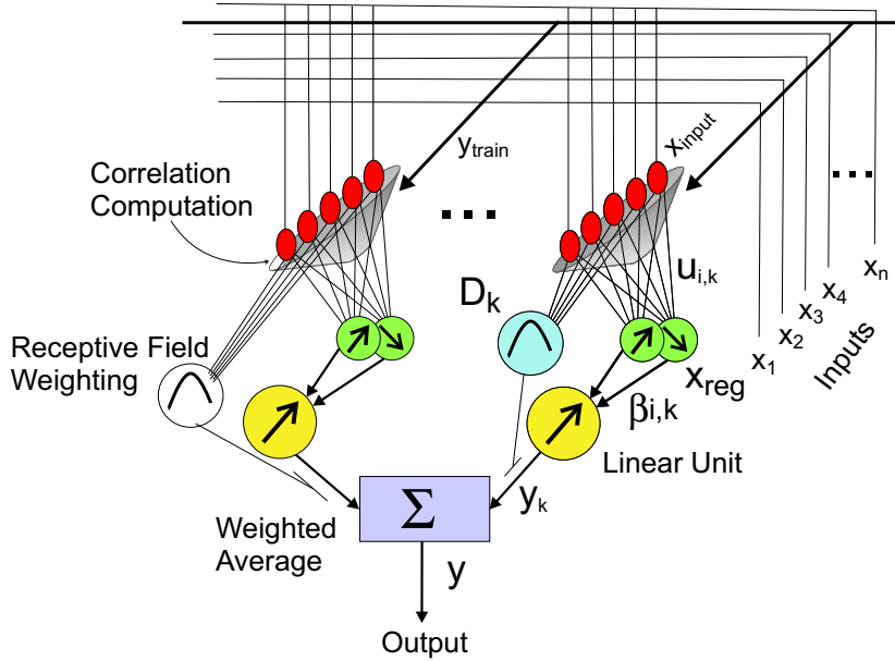
Figure 1: Information processing unit of LWPR
