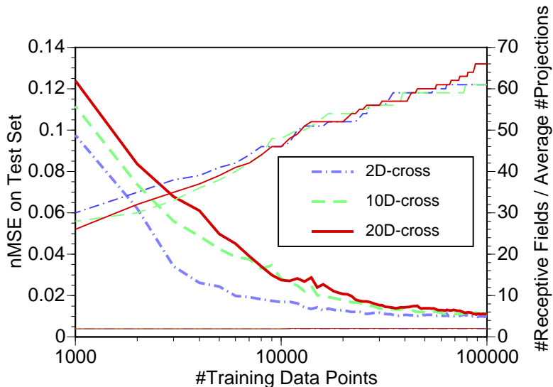
Figure 5: Learning curves for 2-D, 10-D and 20-D data for cross approximation
