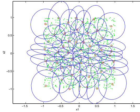
Figure 4: The automatically tuned distance metric for the cross approximation
