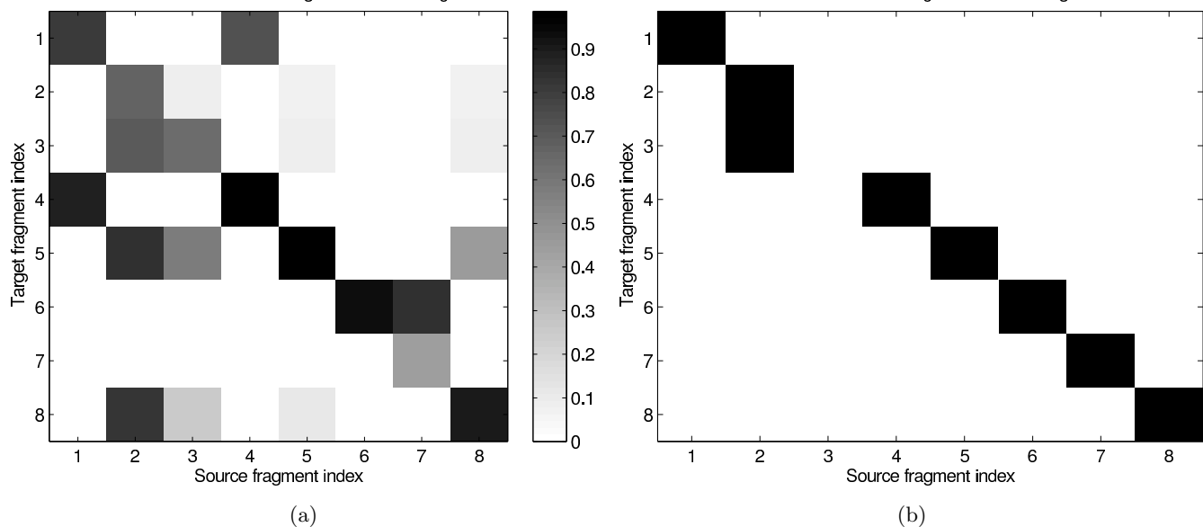
Figure 4: Fragment relatedness experiment in Asia network. (a) The inferred fragment relatedness between target and source fragments. (b) The final selected source fragment for each target.
