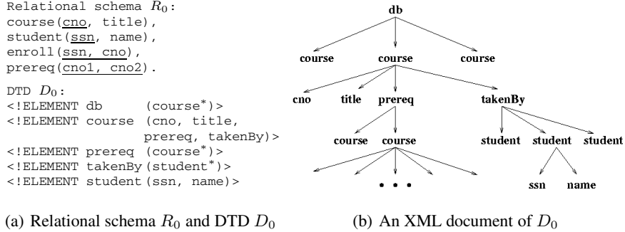
Fig. 1. Relational Schema R_0 , DTD D_0 and an example XML document of D_0
