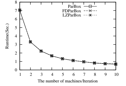
Figure 9: Query q_{F_0}
