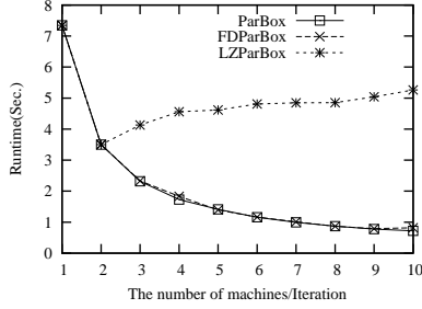
Figure 10: Query q_{F_n}
