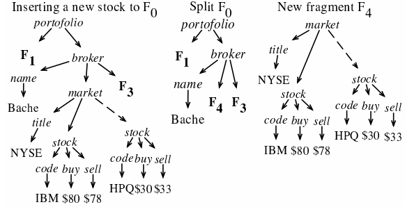
Figure 5: Updates on data and fragments
