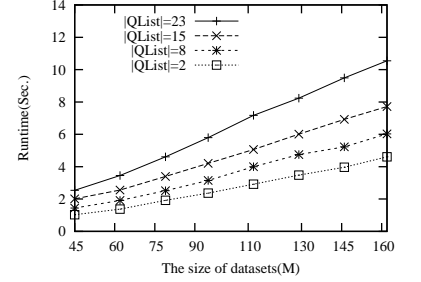
Figure 12: Scalability in data
