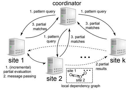
Figure 3: Distributed pattern dependency matching: framework
