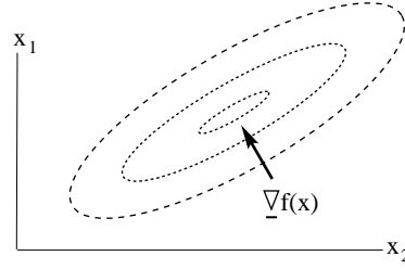
Figure 1: Interpreting the gradient. The ellipses are contours of constant function value, f = \text{const} . At any point \mathbf{x} , the gradient vector \nabla f(\mathbf{x}) points along the direction of maximal increase of the function.
