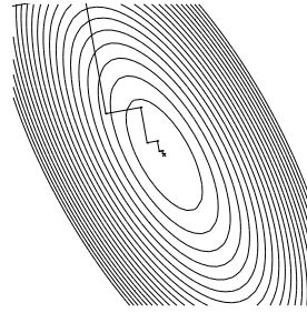
Figure 2: Optimisation using line search along steepest descent directions. Rushing off following the steepest way downhill from a point (and continuing for a finite time in that direction) doesn't always result in the fastest way to get to the bottom!
