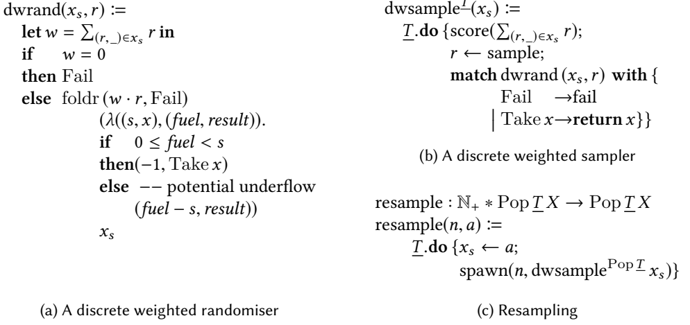
Fig. 10. The resampling transformation
