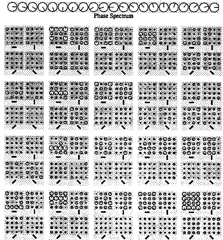
Figure 4: Complex feature-to-hidden connection weights learned by MAGIC. In this simulation, there are connections from a 4 \times 4 patch of the image to a pool of 20 hidden units. (These connections are replicated for each patch in the image to achieve a uniformity of hidden unit response.) The connections feeding into each hidden unit are presented on a light gray background. Each hidden unit has a total of 64 incoming weights— 4 \times 4 locations in its receptive field and four feature types at each location. The weights are further grouped by feature type (dark gray background), and for each feature type they are arranged in a 4 \times 4 pattern homologous to the image patch itself. The area of a circle is proportional to the amplitude of the corresponding weight, the orientation of the internal tick mark represents the phase angle. Due to the symmetry constraint, hidden-to-feature weights (not shown) mirror the feature-to-hidden weights.
