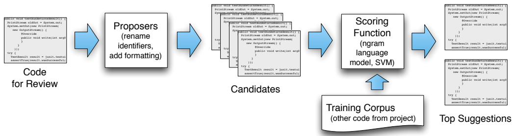
Figure 3: The architecture of NATURALIZE: a framework for learning coding conventions. A contiguous snippet of code is selected for review through the user interface. A set of proposers returns a set of candidates, which are modified versions of the snippet, e.g., with one local variable renamed. The candidates are ranked by a scoring function , such as an n -gram language model, which returns a small list of top suggestions to the interface, sorted by naturalness.
