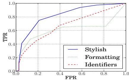
Figure 6: Evaluation of stylish? tool for rejecting unnatural changes. To generate unnatural code, we perturb one identifier or formatting point or make no changes, and evaluate whether NATURALIZE correctly rejects or accepts the snippet. The graph shows the receiver operating characteristic (ROC) of this process for stylish? when using only identifiers, only formatting or both.
