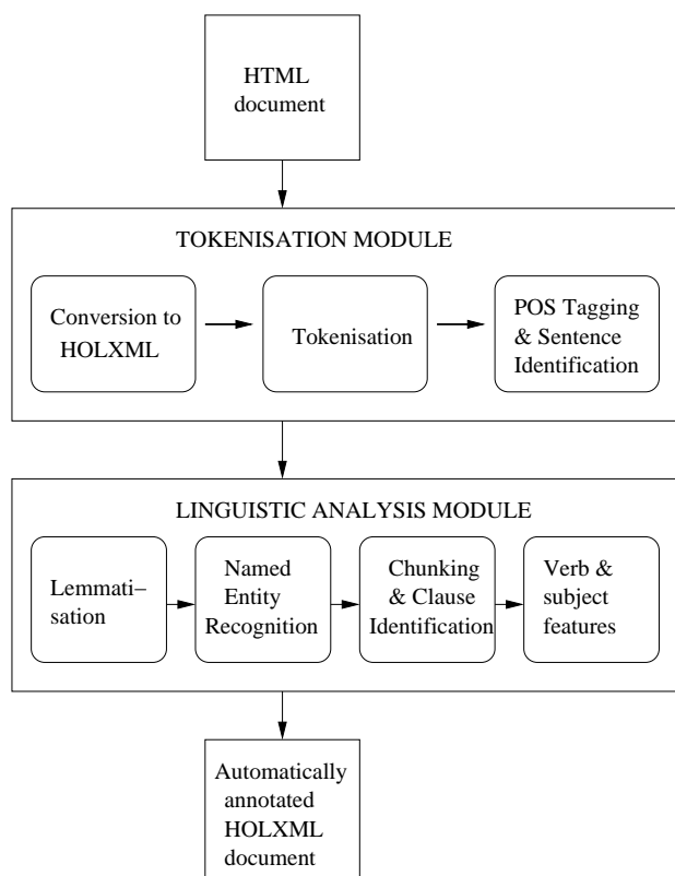
Figure 1. HOLJ Processing Stages
