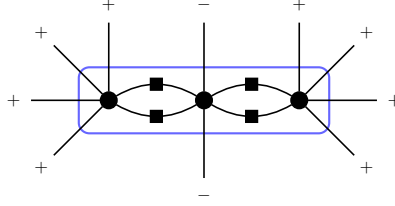
Figure 18: Example E_6 -block. Circle vertices are assigned =_6 and square vertices are assigned \neq_2 .
