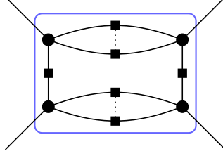
Figure 23: Gadget to realize \hat{g} in Lemma 7.10. Circle vertices are assigned =_k and square vertices are assigned \neq_2 . The number of parallel edges is k - 2 .
