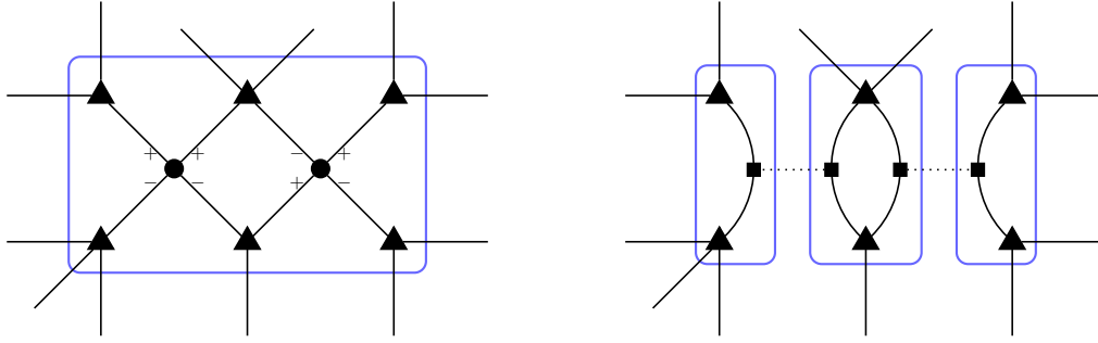
(a) An EO-Eq-4 -block. Triangles are assigned EXACTONE signatures and circles are E_k -blocks of arity 4.
