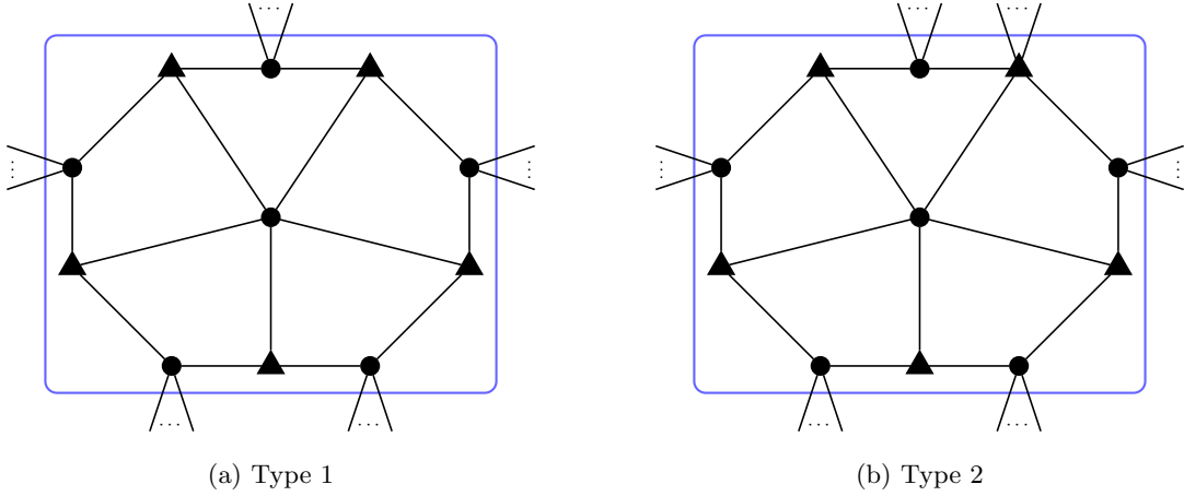
Figure 21: Two types of wheels. Each circle is an E_5 -block and triangle an EXACTONE signature.
