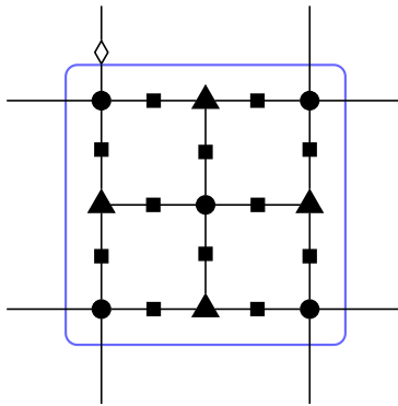
Figure 16: Grid-like gadget used in the proof of Lemma 7.3, whose support vectors are 00110011, 11001100, and 11111111. Each square is assigned a binary disequality \neq_2 , circle =_4 , and triangle [0, 1, 0, 0] .
