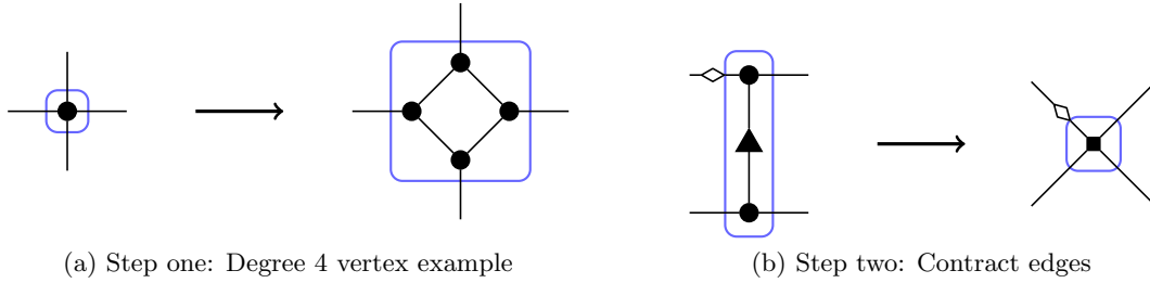
Figure 14: A reduction from Pl-Holant( \mathcal{EQ} \mid h ) to Pl-Holant( g ) for any binary signature h and a quaternary signature g that depends on h . The circle vertices are assigned =_4 or =_3 respectively, the triangle vertex is assigned h , and the square vertex is assigned the signature of the gadget to its left.
