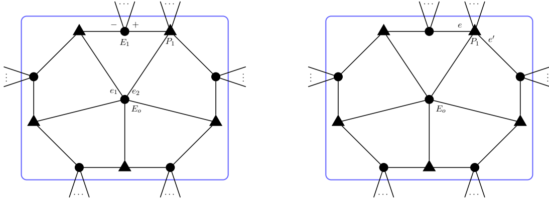
(a) Different signs of an E_5 -block along the cycle lead to pinning
