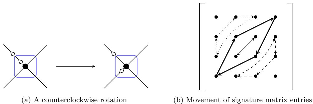
Figure 2: The movement of the entries in the signature matrix of a quaternary signature under a counterclockwise rotation of the input edges. Entries of Hamming weight 1 are in the dotted cycle, entries of Hamming weight 2 are in the two solid cycles (one has length 4 and the other one is a swap), and entries of Hamming weight 3 are in the dashed cycle.
