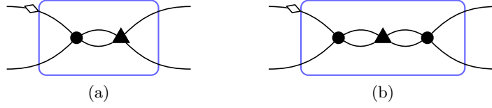
Figure 32: Two gadgets used in the proof of Lemma F.4.
