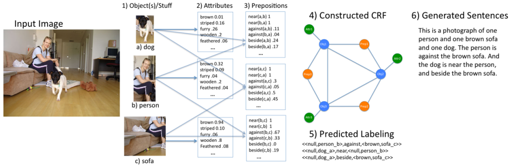
Figure 1: The automatic image description generation system proposed by Kulkarni et al. (2011).
