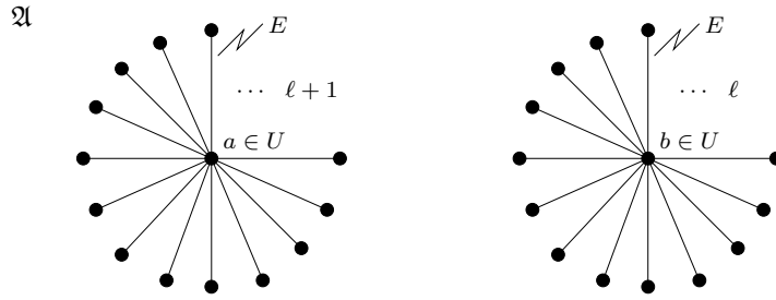
Figure 1: Structure \mathfrak{A} of Example 1.1.
