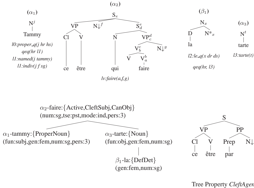
Derivation Tree
