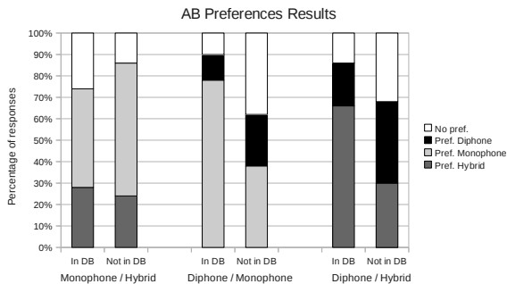
Figure 2: Results for AB comparison test. For proper names in the database, there is a significant preference for the monophone and hybrid systems over the diphone one. For proper names outside the database, there is a significant preference for the monophone system over the hybrid one.
