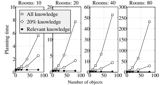
Figure 4: Planning time with PA scales well to larger number of rooms and objects (Zhang et al. 2014).
