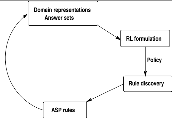
Figure 2: The closed loop of knowledge representation and reinforcement learning enables discovery of new rules and their use in subsequent inference.
