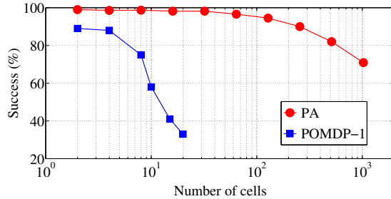
Figure 3: With a limit on the policy computation time, PA significantly increases accuracy in comparison with just POMDPs as the number of cells increases (Zhang et al. 2014).
