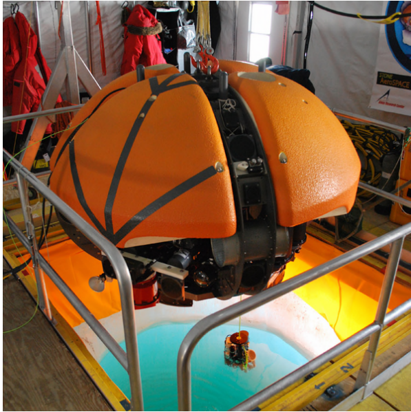
Figure 1: ENDURANCE in position over the Lake Bonney deployment melt hole. The drop sonde can also be seen suspended below the vehicle in a partially deployed position as part of the instrument calibration.
