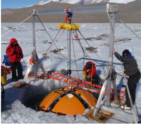
Figure 6: ENDURANCE surfaced at secondary melt hole in preparation for ballasting for sub-halocline operations.
