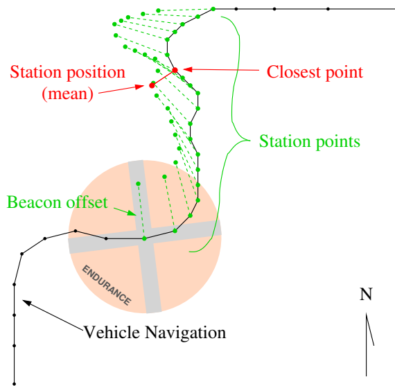
Figure 11: Example of station definition for ice picking. The dead-reckoned measurements of the vehicle trajectory are shown in black. The points chosen to define the station are in green, along with the position of the magnetic beacon (offset from the vehicle center), which is the actual point measured by the GPS fixes. In this example, upon reaching the target location, the vehicle drifts for some time before vertical motion (out of the plane of the figure) ceases and ice picking is determined to have started. During the course of the picking and obtaining the magnetic beacon fix ( \sim 1-5 min), the vehicle skids slowly along the ice roof before diving and resuming its course eastward toward the next waypoint. The actual station position is the position that would be measured with a GPS magnetic beacon fix, shown in red. For ice-picking, this is assumed to be the mean of the beacon position during the episode. The uncertainty in the measurement includes the spread in the station points. Also in red is the closest point on the dead-reckoned vehicle trajectory. The absolute measurement update of is applied to this point.
