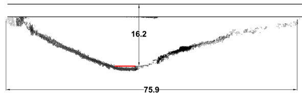
Figure 14: Cross-section of bathymetry at historical minimum width of the Narrows. Scott's measurement is shown in red, at the resulting required depth relative to the modern lake level of 16.2 m.
