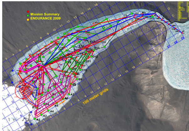
Figure 5: Summary view of all 2009 ENDURANCE mission trajectories.
