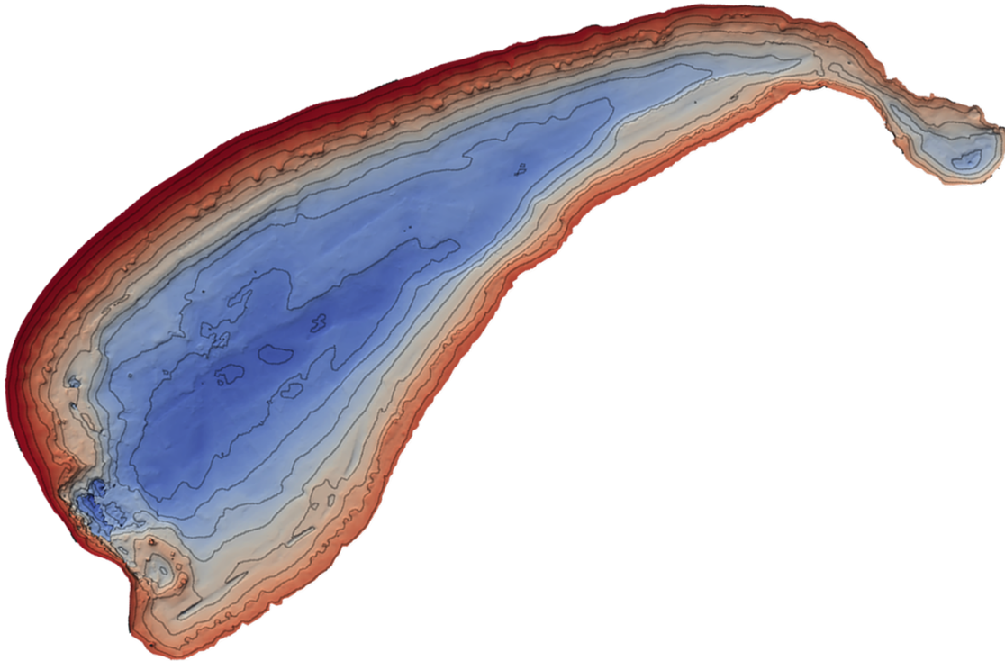
Figure 13: The final mesh generated through poisson reconstruction contained about 500 000 vertices and 800 000 faces.
