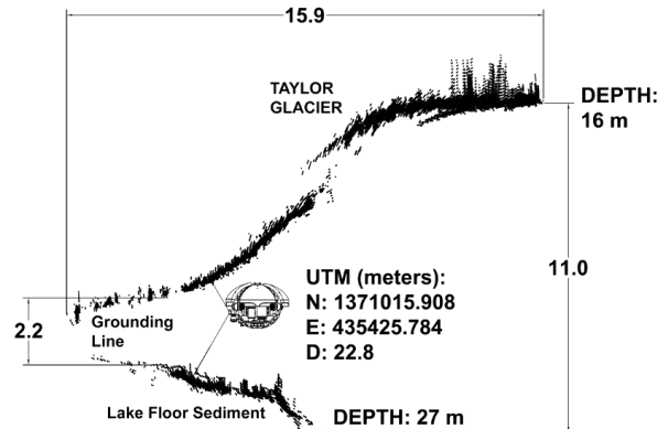
Figure 7: Schematic view of sub-halocline exploration, including raw multi-beam sonar data. The overhanging ledge of glacier ice is visible at top-right at a depth of 16 m (cf. Fig. 3). Due to the limited clearance, ENDURANCE was unable to fully penetrate to and image the glacier grounding line, but was able to establish its depth and general geometry using the multi-beam sonar.
