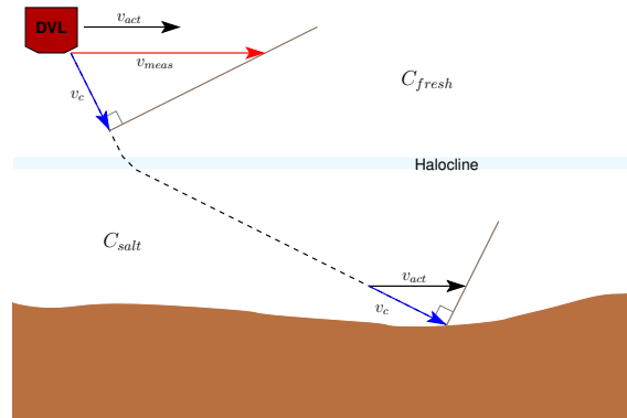
Figure 10: Additional DVL scale error introduced by Lake Bonney environment: schematic of one DVL sonar beam. The actual DVL velocity is v_{act} . The Doppler shift in the beam is induced by the velocity component v_c along the (bent) beam at the lake bottom. This in turn causes the velocity v_{meas} derived at the DVL transducer and based on the outgoing beam angle to be scaled.
