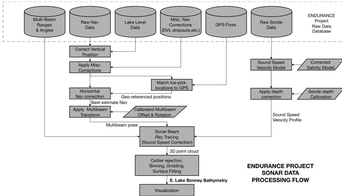
Figure 8: ENDURANCE sonar bathymetry data processing flow.
