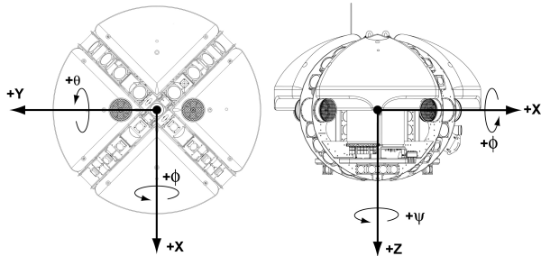
Figure 4: Schematic of ENDURANCE vehicle indicating vehicle axes.
