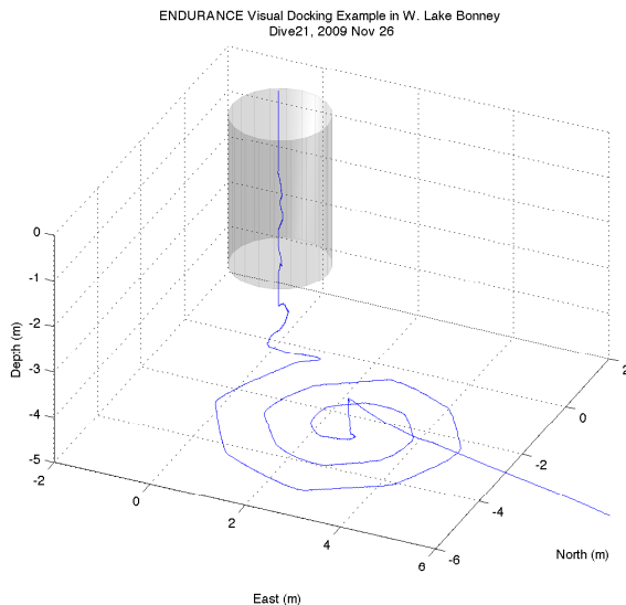
Figure 9: Example of autonomous visual docking at the deployment melt hole (represented by the gray cylinder). The vehicle trajectory is indicated by the blue trace. The vehicle arrives at the presumed location of the melt hole, which, due to navigation errors, is not the true location. It begins an outward spiral search until identifying the blinking light in the upward-looking camera. It then centers on the light and moves up the melt hole to be recovered.
