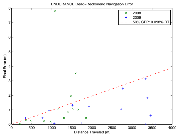
Figure 12: Actual dead-reckoning performance of ENDURANCE vehicle in Lake Bonney, based on error at return to deployment melt hole. The 50% circular error probable (CEP), assuming symmetric binormal distribution of position errors, is 0.098% of distance traveled.
