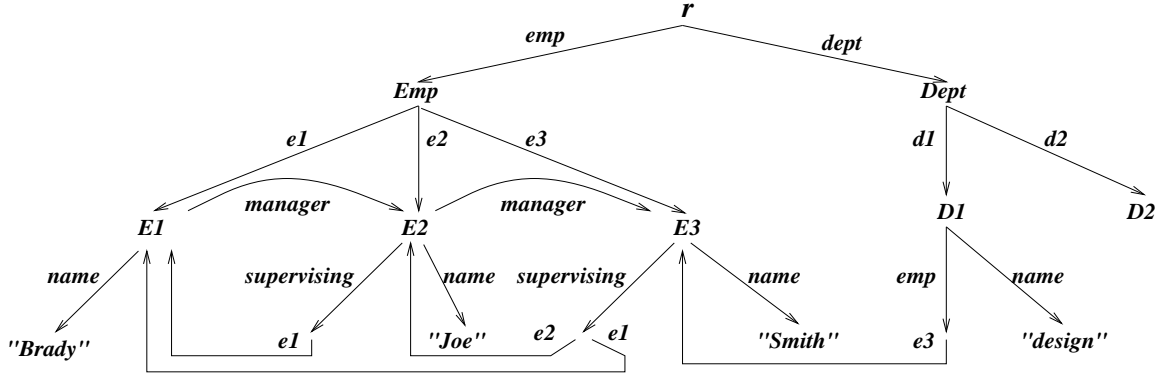
Figure 1: An example semistructured database in DM
