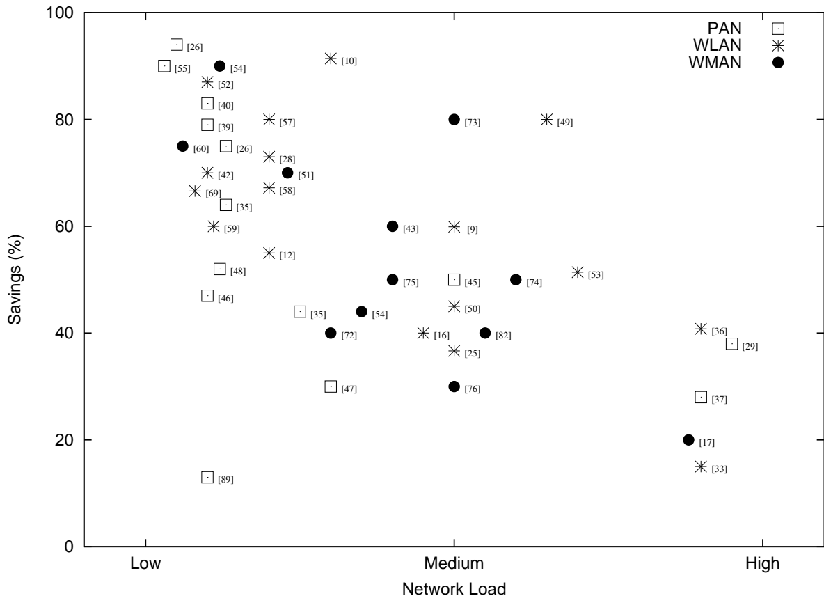
Figure 3: Typical savings achieved depending on the network load.
