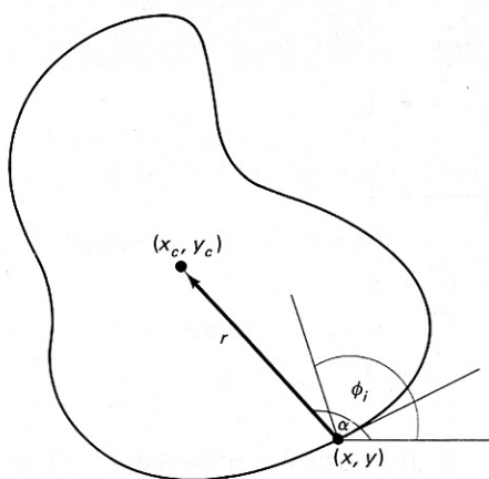
Fig. 4.8 Geometry used to form the R -Table.
