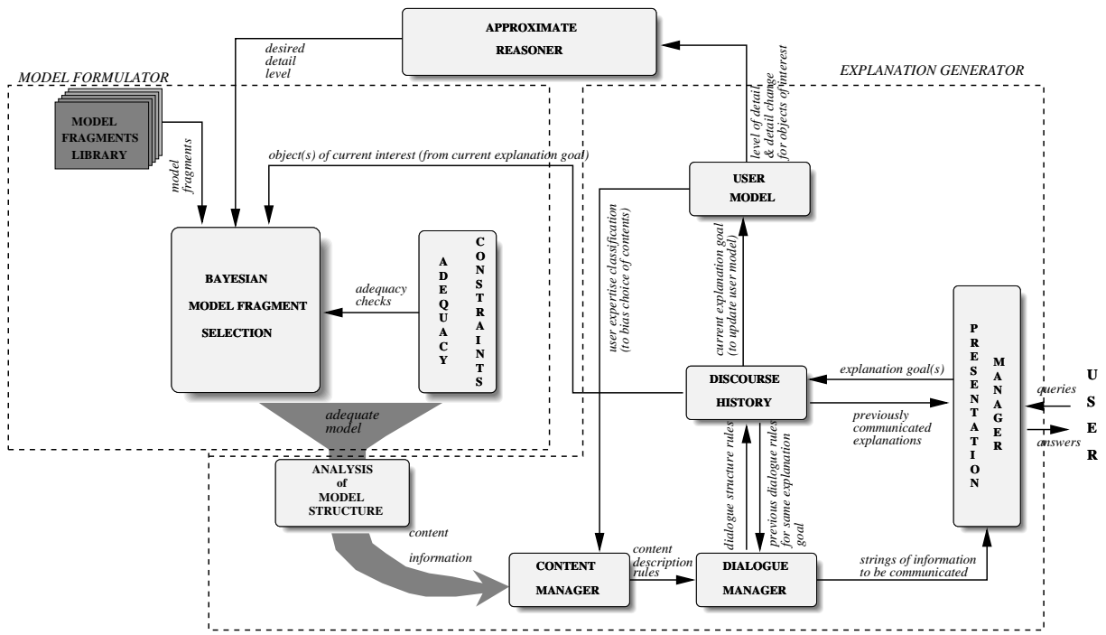
Figure 1: Explanation system : individual modules and their components
