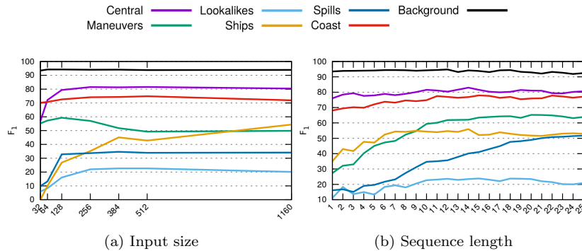
Figure 6: Comparison of the result obtained for each of the classes when varying: (a) The input size of the CMSAE networks and (b) the number of scanlines used as input. See Table 5 for standard deviation of results based on the settings shown in Table 2.
