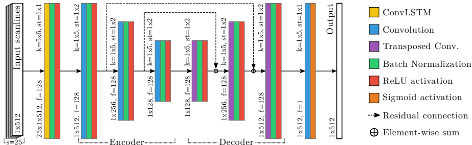
Figure 4: Scheme of the CMSAE network specialized for the segmentation of oil spills. In this figure, the layer type is labeled with colors according to the side legend. The size of each layer for convolutions and transposed convolutions is h \times w , where h is the height and w the width. The size for the ConvLSTM layer is s \times h \times w , where s is the sequence length. The number of filters ( f ), the kernel size ( k ) and the stride value ( st ) applied for each layer are also shown. The CMSAE networks used for the segmentation of the other classes follow the same scheme, although their topologies vary.
