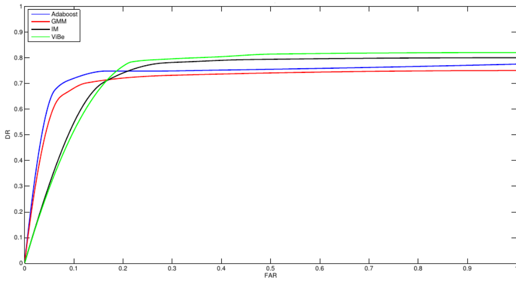
Figure 11: ROC curve for the motion detection algorithms used in this work.
