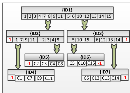
Figure 5: A Balance-guaranteed Optimized Tree computed from training data is shown, where the leafnodes contain classifiers that either separate the fish in more subclasses or reject the fish for a particular subnode (shown by the “-1” branch), because it is not similar to the fish species in that particular node. Rejected fish are classified by a flat Support Vector Machine in this case.
