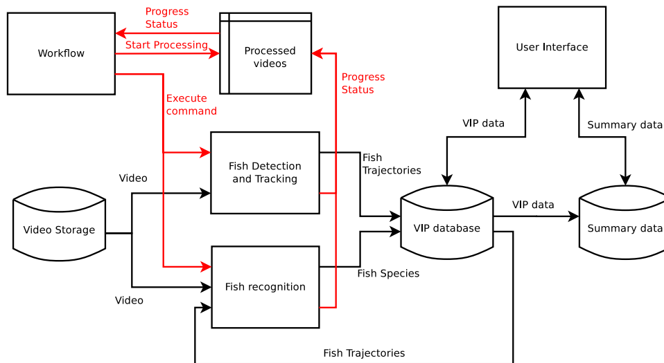
Figure 3: Schematic overview of the research tool for analysing fish assemblages with video data. The black arrows show the dataflow in the system, while the red arrows show the workflow of the system. This system finds the “fish trajectory” (positions of single fish in the multiple frames) in the video and given the fish trajectories determines the most likely fish species. This information is all stored in a Video/Image Processing (VIP) database. The user interface queries the summary data from this VIP database allowing marine ecologists to analyse this information.
