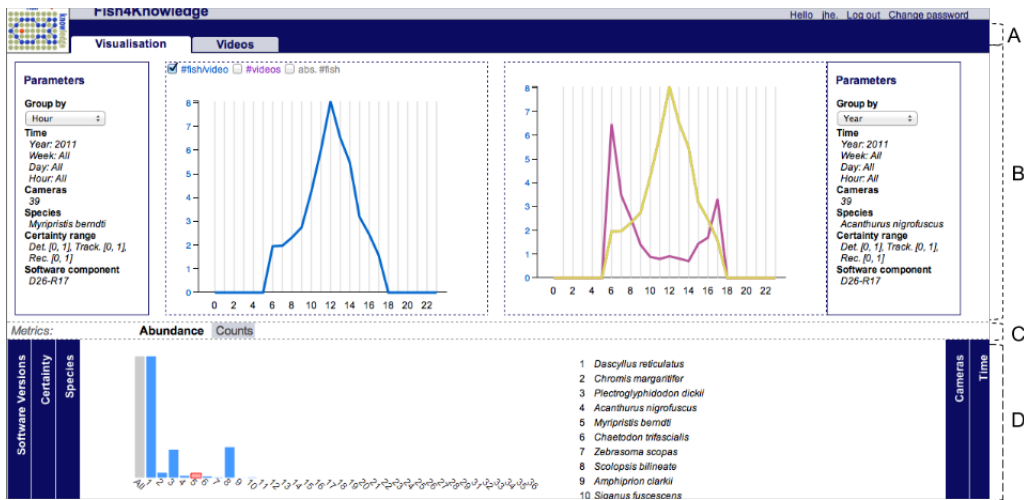
Figure 7: An overview of the user interface, in the “visualization” view.
