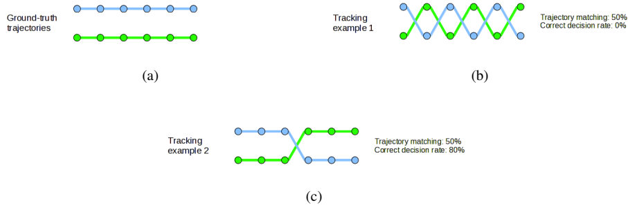
Figure 12: Fig. 12(a) shows two ground truth trajectories of two fish, whereas the other two images represent two examples of tracking output. In Fig.12(b), although the tracker fails at each tracking decision the average trajectory matching score is 50%, whereas the correct decision rate is 0%. In Fig. 12(c) the tracker fails only in one step and the average trajectory matching score is 50% (as the previous case) whereas the correct decision rate is 80% (4 correct associations out of 5).
