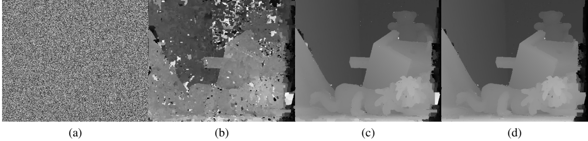
Figure 5: Proposed algorithm with random initialization ( \tau_{grad} = 5/255 , \tau_{cen} = 5/25 , and no multi-scale), intermediate and final results: (a) Initial random configuration; (b) First propagation, E = 123,257.02 ; (c) First Refinement, E = 87,134.61 ; (d) Final Result, E = 82,334.98 .
