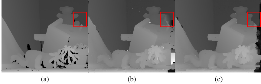
Figure 3: Raw result of Teddy image ( \tau_{grad} = 5/255 , \tau_{cen} = 5/25 , random initialization, and no multi-scale). (a) Groundtruth Teddy image; (b) Uniqueness term is disabled; (c) Uniqueness term is enabled.
