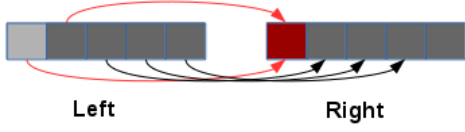
Figure 2: Example of uniqueness constraint violation; two pixels (red arrows) in left image scanline map to a single pixel in right image (red pixel).
