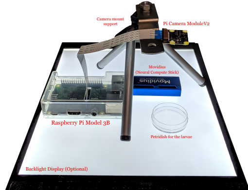
Figure 1: Proposed image acquisition system: The system includes a Raspberry Pi (model 3B) combined with a Pi camera module v2 for video imaging as well as an Intel Movidius Neural Compute Stick for tracking with a deep-learning based system. Though the back light display is optional, uniform lighting enhances video quality and potentially enables the presentation of stimuli for psychophysics studies.
