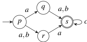
(b) GFP is not closed under union: Pruning automaton \mathcal{A} with P(id, \sqsubseteq^{di}) \cup P(\sqsubseteq^{bw}, id) would remove the transitions p \xrightarrow{a} r and q \xrightarrow{a} s , and thus aac^\omega would no longer be accepted.
