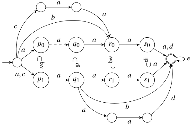
(a) P(\sqsubseteq^{bw}, \sqsubseteq^{di}) is not GFP: If the dashed transitions p_0 \xrightarrow{a} q_0 and r_1 \xrightarrow{a} s_1 are removed, then a^5 e^\omega is no longer accepted. Note that \mathcal{A} = \mathcal{A} / \sqsubseteq^{bw} = \mathcal{A} / \sqsubseteq^{di} . (This example even holds for \prec^{k-bw}, \prec^{k-di} and k = 3 ; cf. Section 4).
