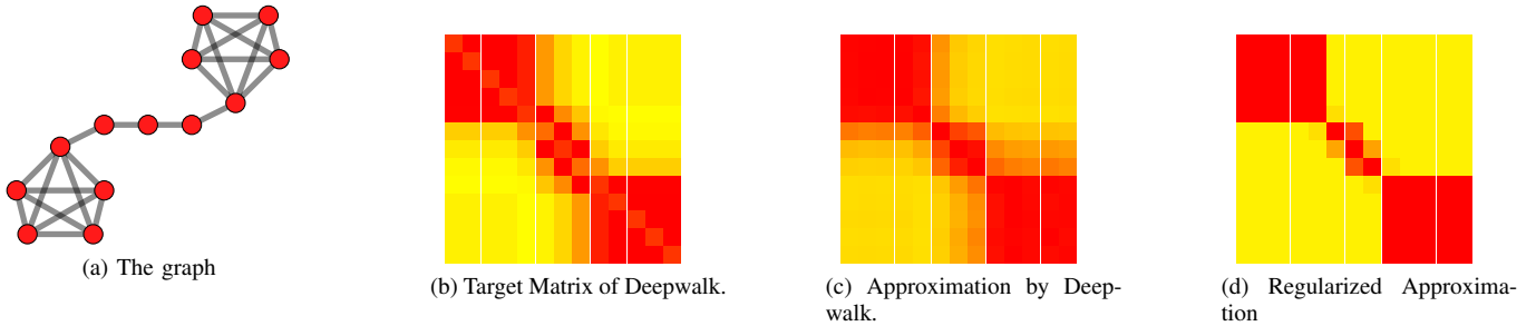
Fig. 3. An example Barbell graph with the corresponding target matrix factorized (window size of 3) by DeepWalk [26] and the reconstructed target matrices obtained with standard DeepWalk and Smooth DeepWalk . Regularized optimization produces more well defined communities. While the standard DeepWalk model has less well defined clusters.
