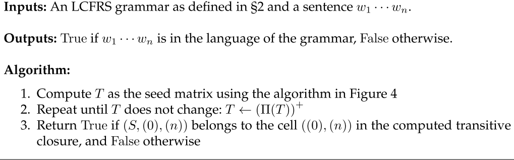
Figure 9 Algorithm for recognizing binary LCFRS when Condition 4.1 is not necessarily satisfied by the LCFRS.
